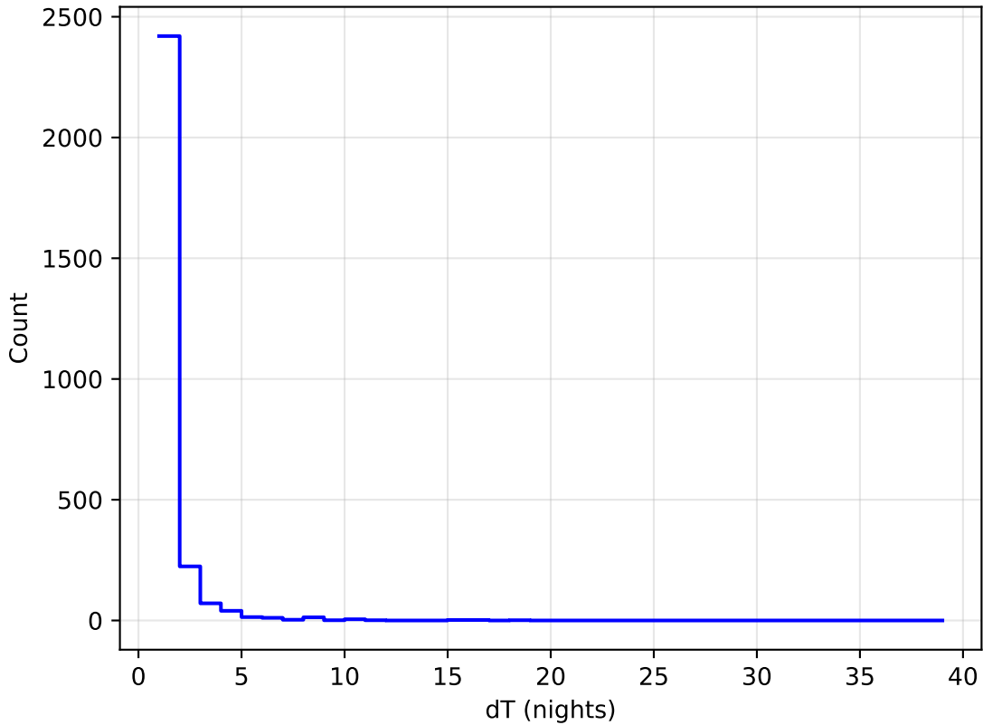
internal_u_expt27_nscale0.9v3.4_10yrs all bands: DD:WFD Delta Nights Histogram
