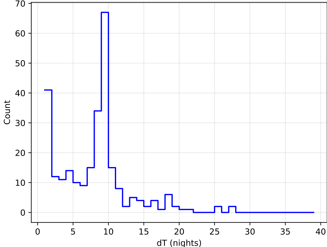
internal_u_expt27_nscale0.9v3.4_10yrs all bands: DD:ELAISS1 Delta Nights Histogram
