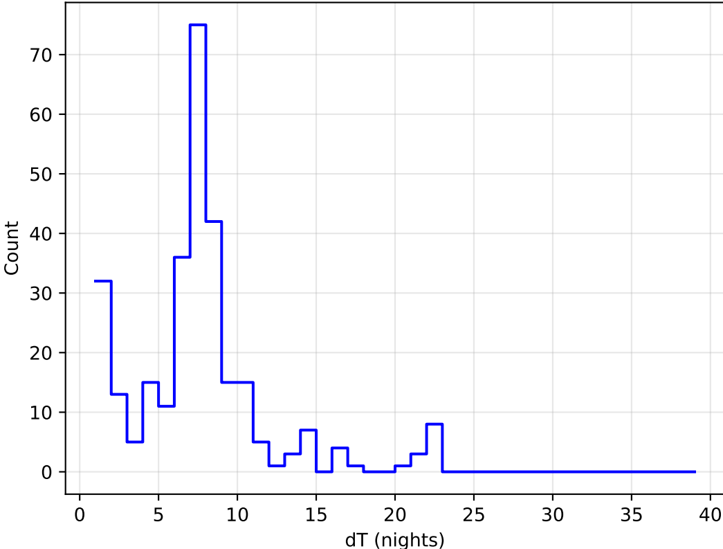
internal_u_expt27_nscale0.9v3.4_10yrs all bands: DD:EDFS Delta Nights Histogram
