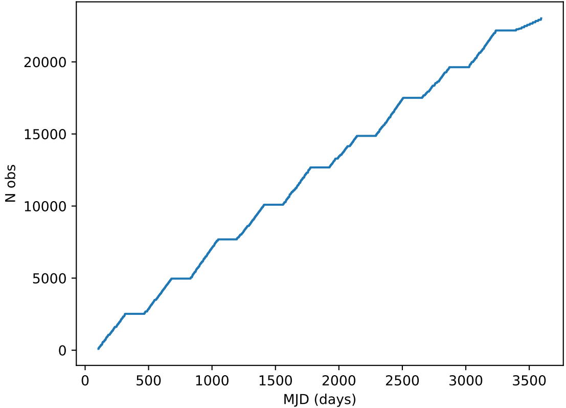
internal_u_expt27_nscale0.9v3.4_10yrs all bands: DD:EDFS Cumulative NVisits
