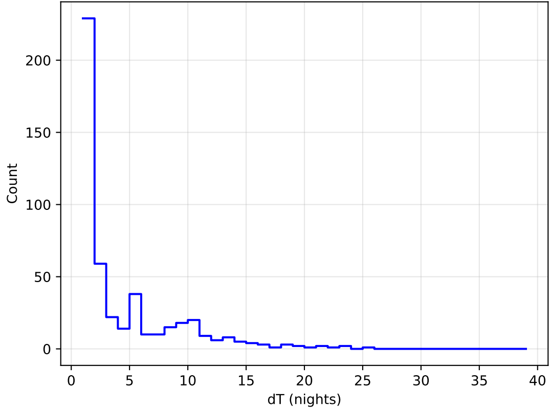
internal_u_expt27_nscale0.9v3.4_10yrs all bands: DD:COSMOS Delta Nights Histogram
