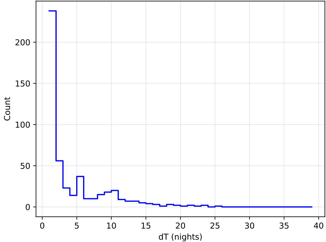
internal_u_expt27_nscale0.9v3.4_10yrs all bands: DD: COSMOS Delta Nights Histogram
