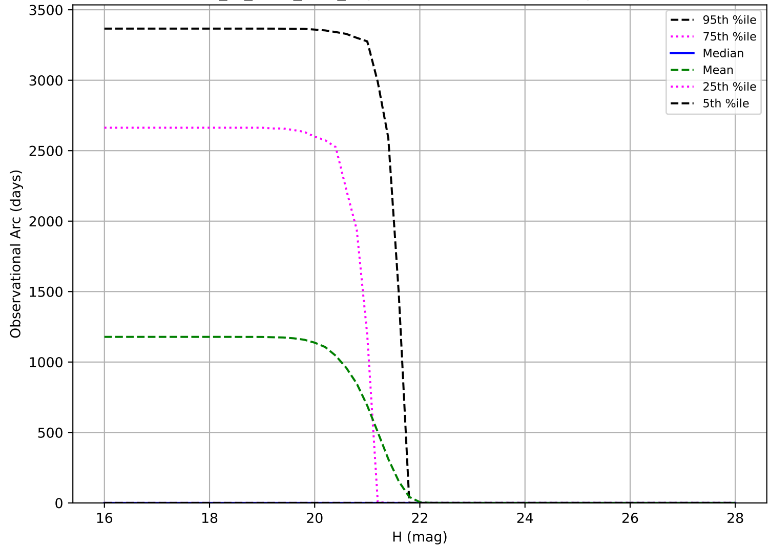
extra_ss_neo7_v3.4_10yrs: Observational Arc Length Vatira
