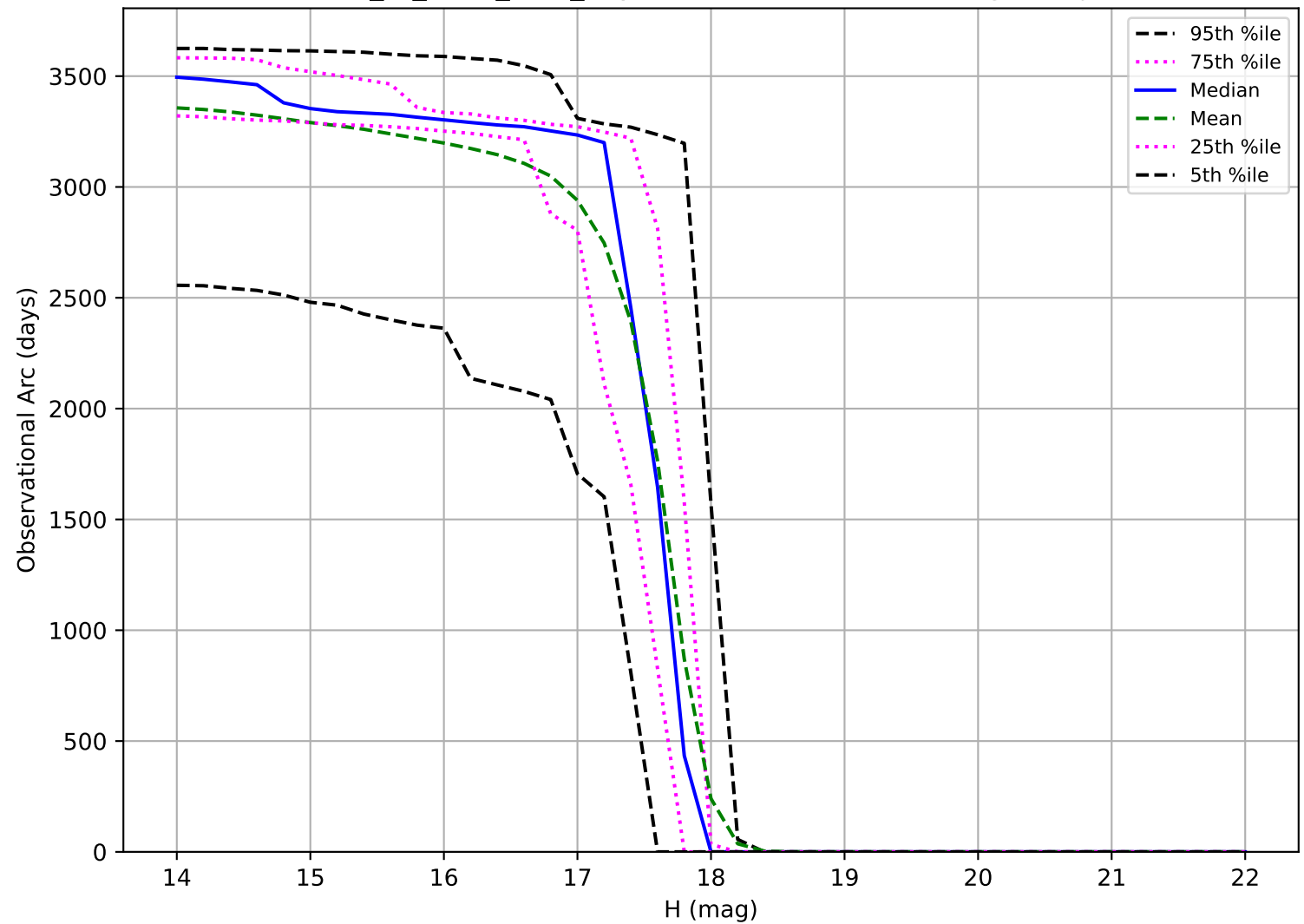
extra_ss_neo7_v3.4_10yrs: Observational Arc Length Trojan
