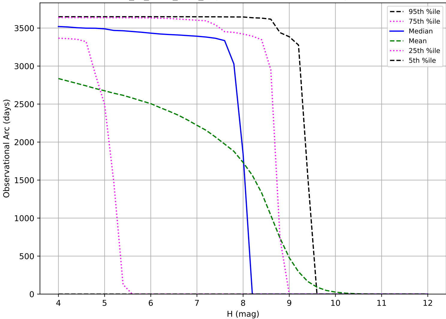
extra_ss_neo7_v3.4_10yrs: Observational Arc Length TNO
