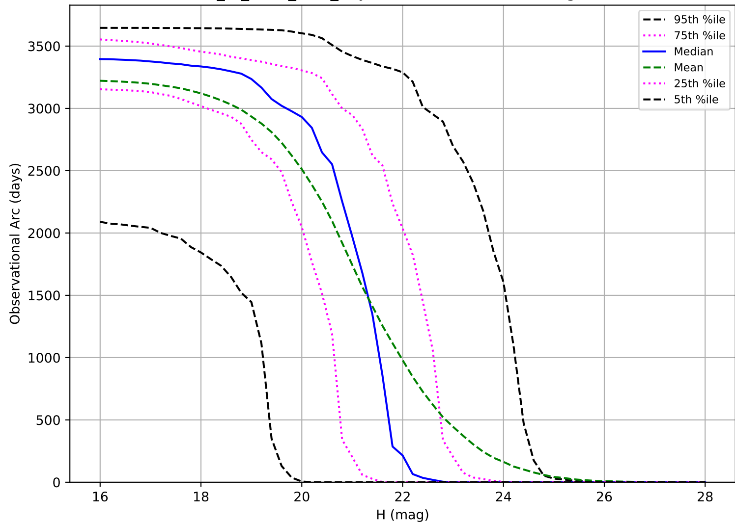
extra_ss_neo7_v3.4_10yrs: Observational Arc Length PHA
