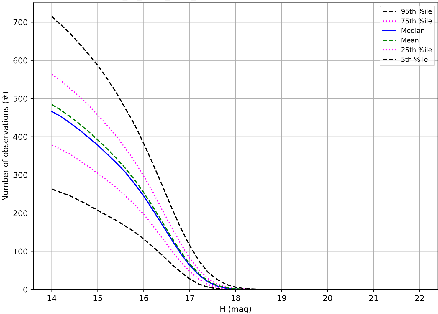
extra_ss_neo7_v3.4_10yrs: Number of observations Trojan
