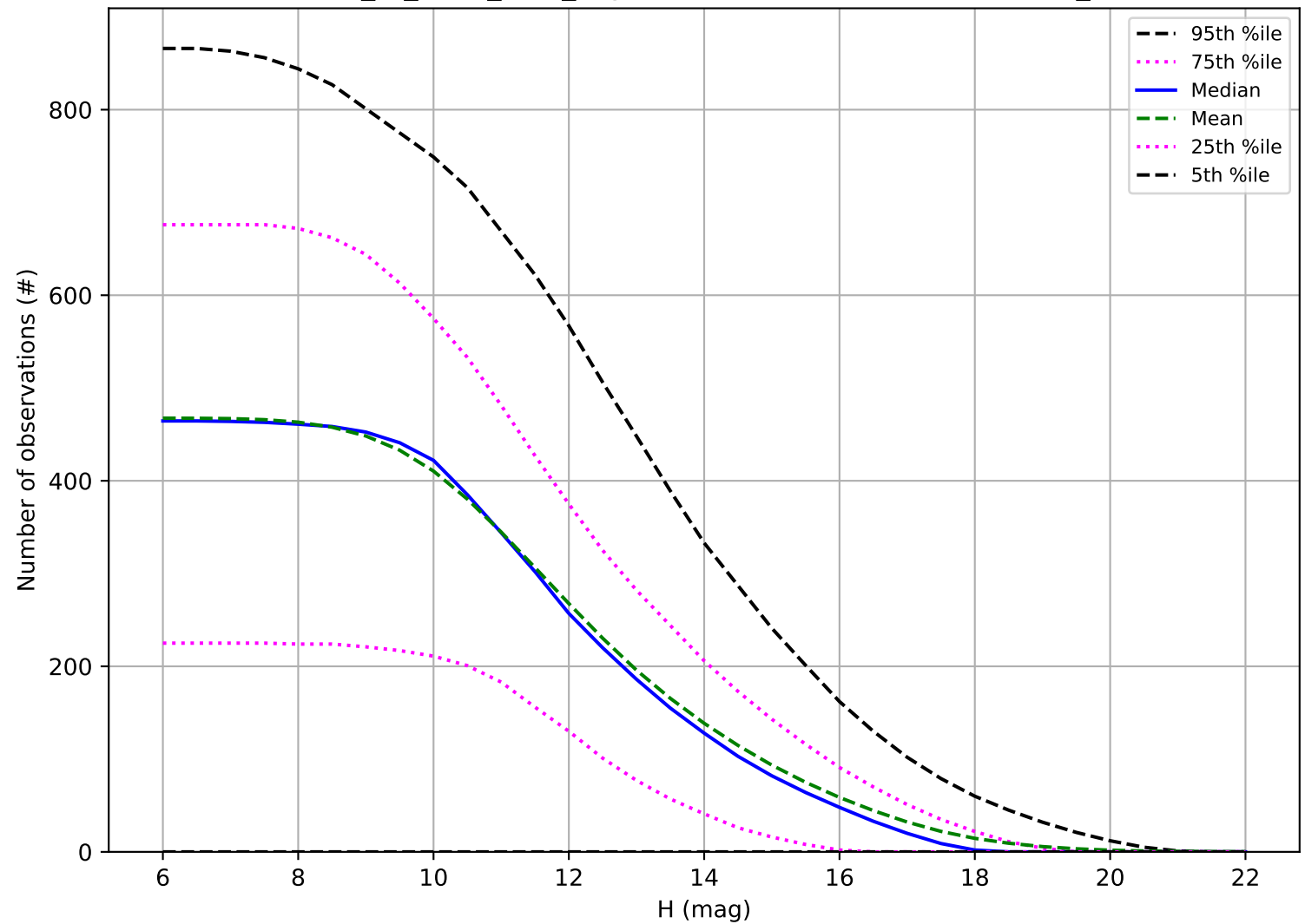
extra_ss_neo7_v3.4_10yrs: Number of observations OCC_r5
