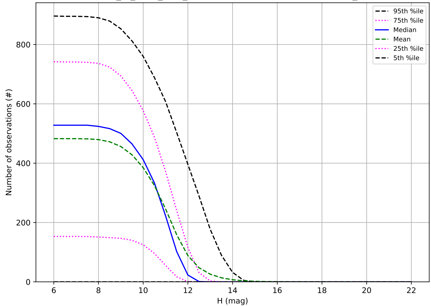
extra_ss_neo7_v3.4_10yrs: Number of observations OCC_r20
