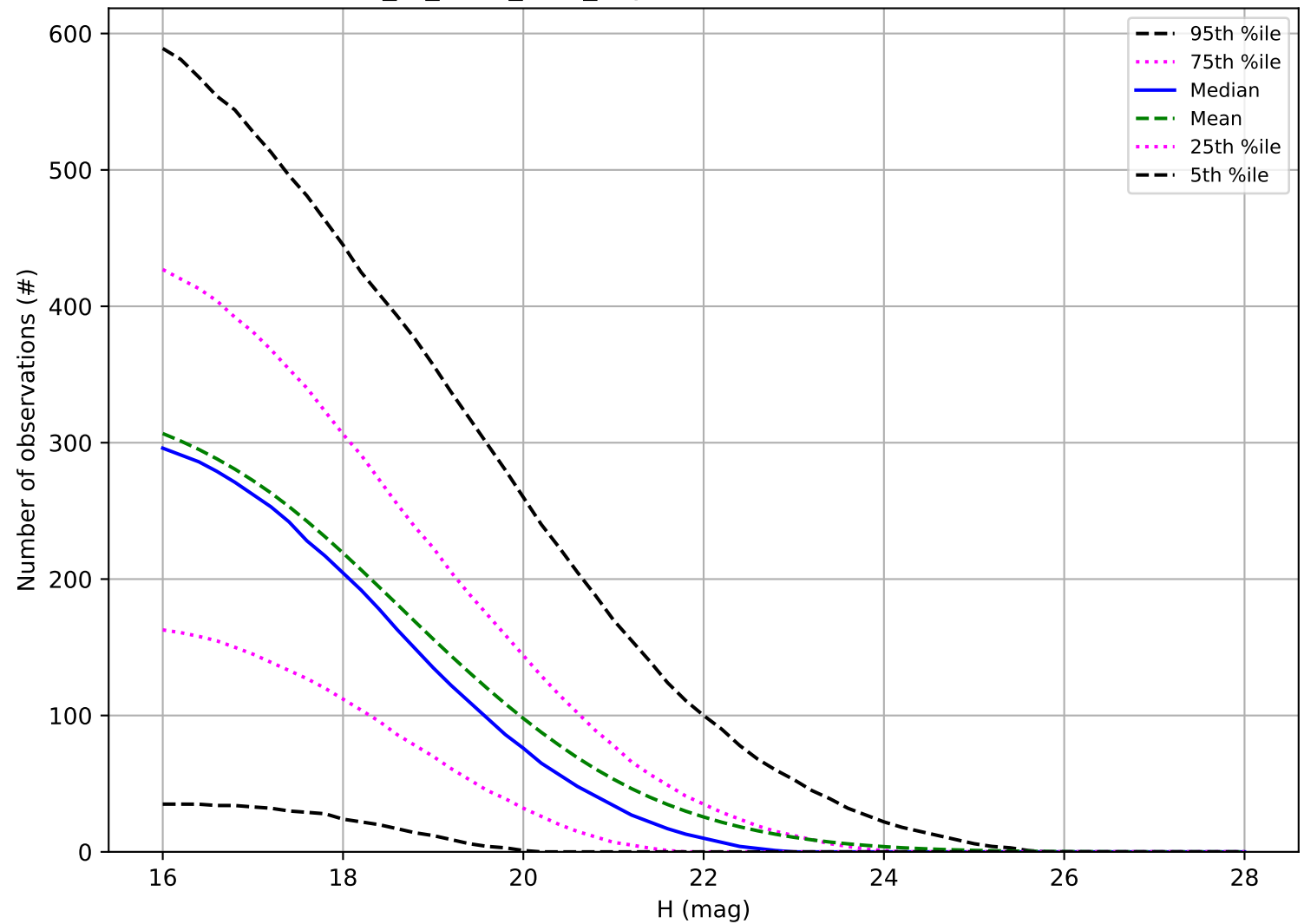
extra_ss_neo7_v3.4_10yrs: Number of observations NEO
