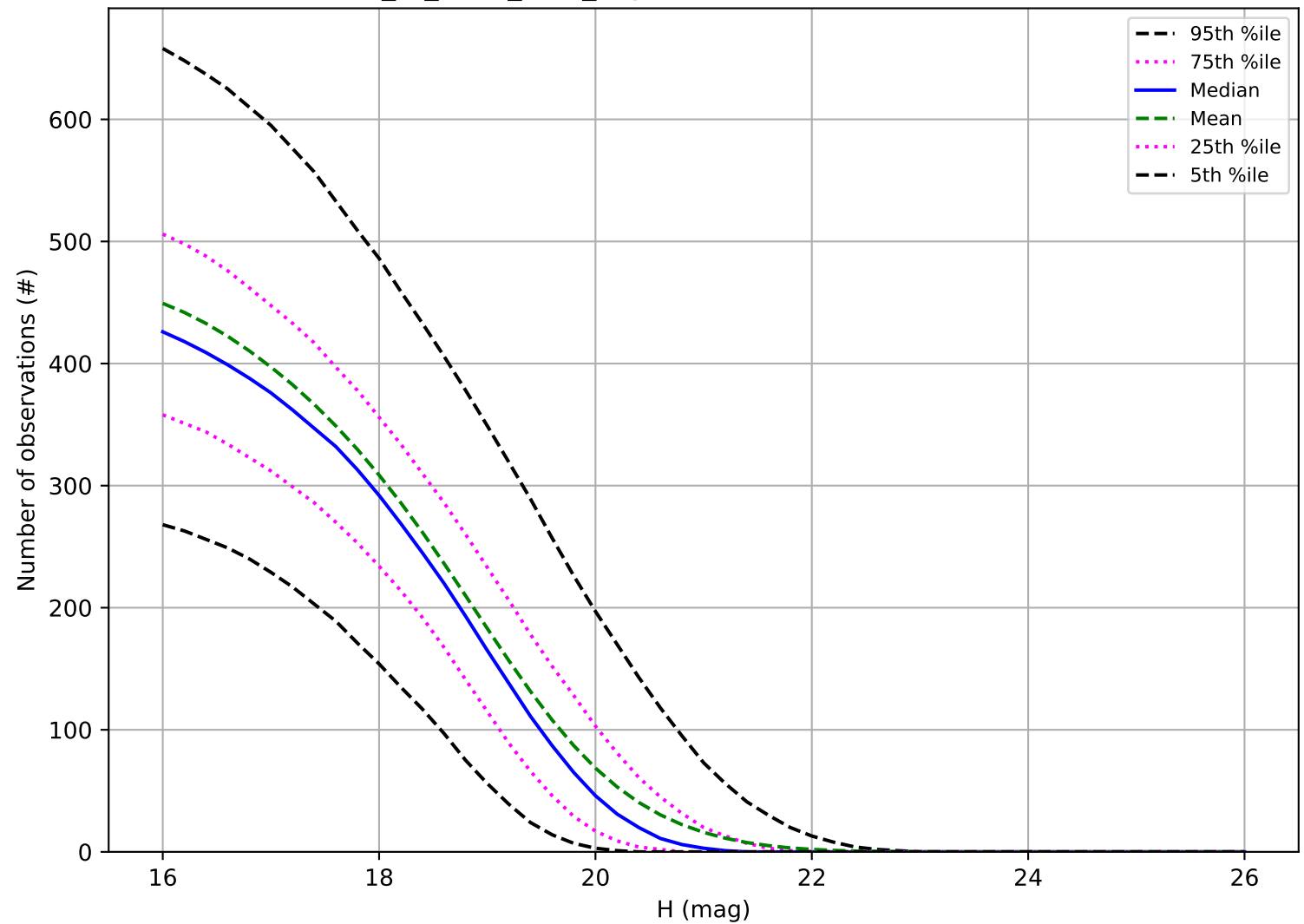
extra_ss_neo7_v3.4_10yrs: Number of observations MBA
