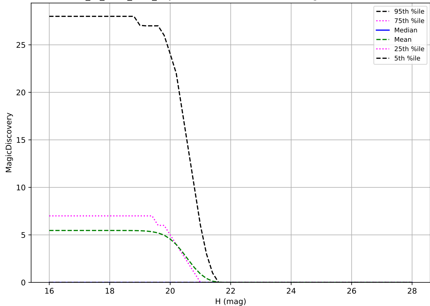
extra_ss_neo7_v3.4_10yrs: Vatira 6 detections in 60 nights detection loss
