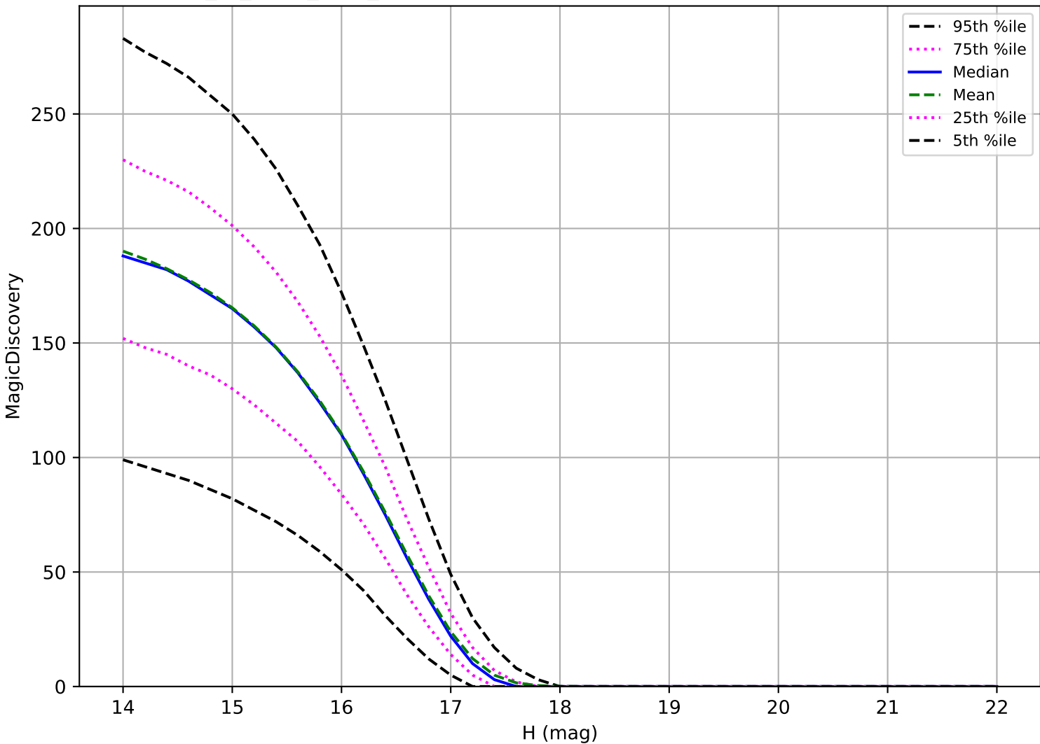
extra_ss_neo7_v3.4_10yrs: Trojan 6 detections in 60 nights detection loss
