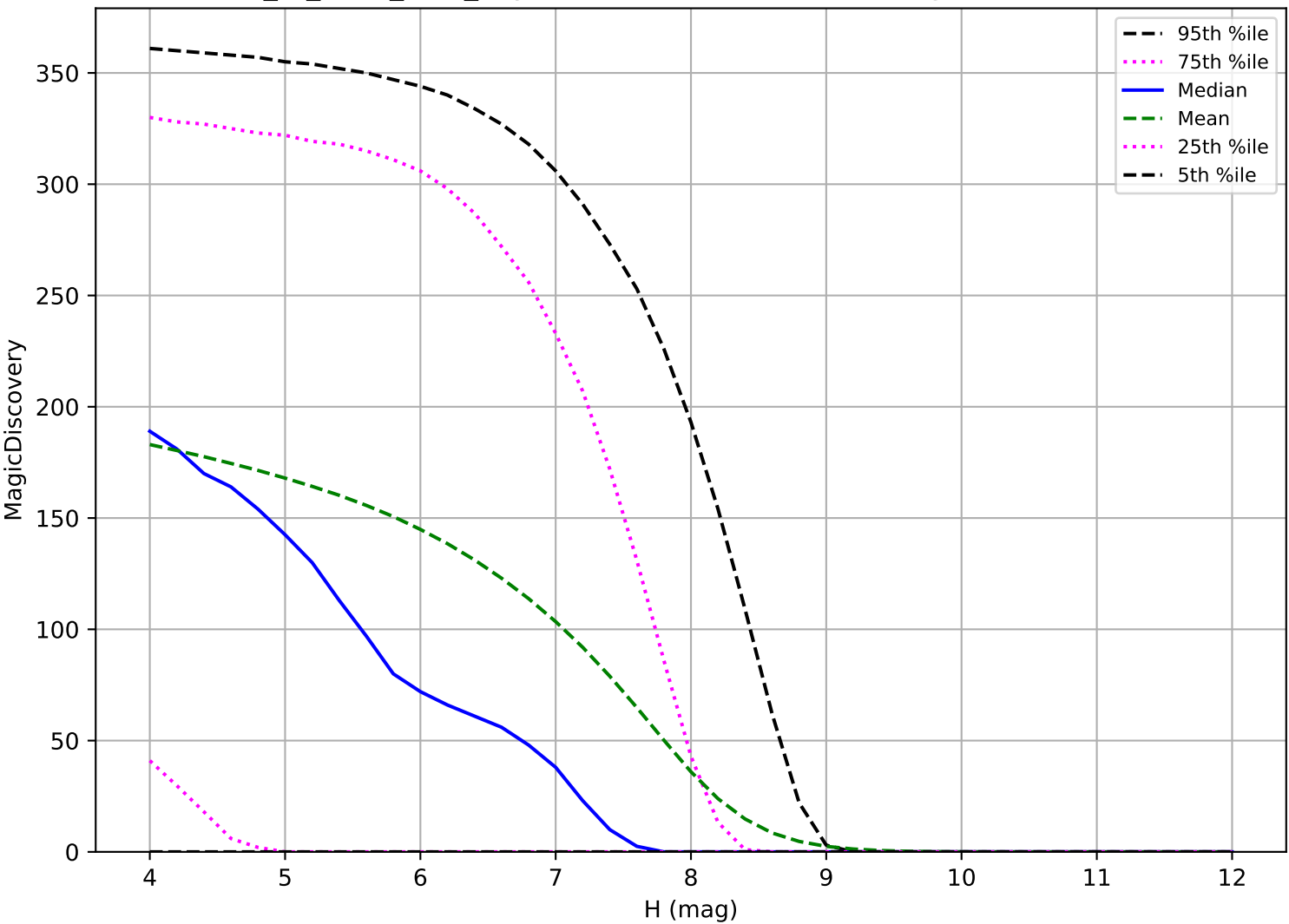
extra_ss_neo7_v3.4_10yrs: TNO 6 detections in 60 nights detection loss
