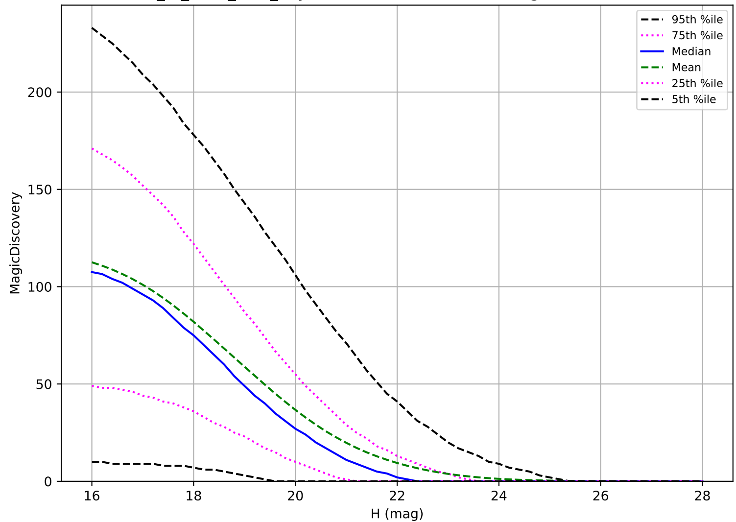
extra_ss_neo7_v3.4_10yrs: PHA 6 detections in 60 nights detection loss
