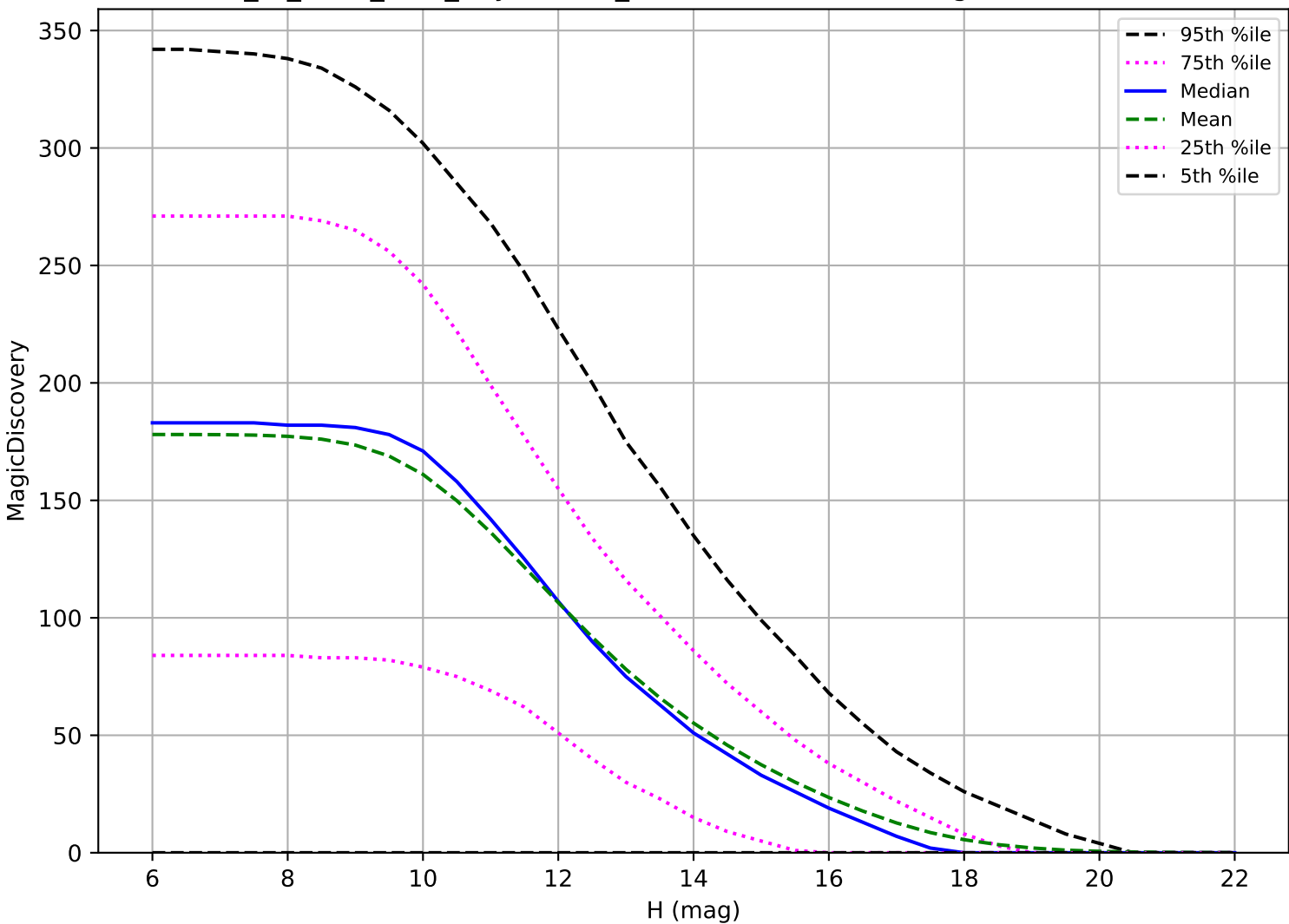
extra_ss_neo7_v3.4_10yrs: OCC_r5 6 detections in 60 nights detection loss
