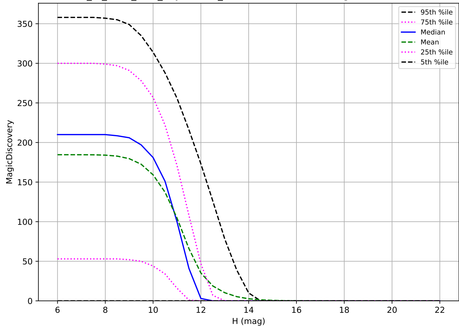
extra_ss_neo7_v3.4_10yrs: OCC_r20 6 detections in 60 nights detection loss
