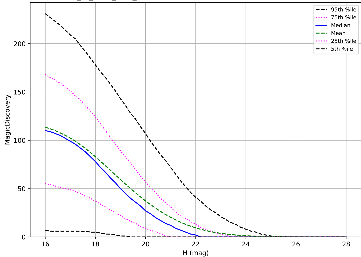
extra_ss_neo7_v3.4_10yrs: NEO 6 detections in 60 nights detection loss
