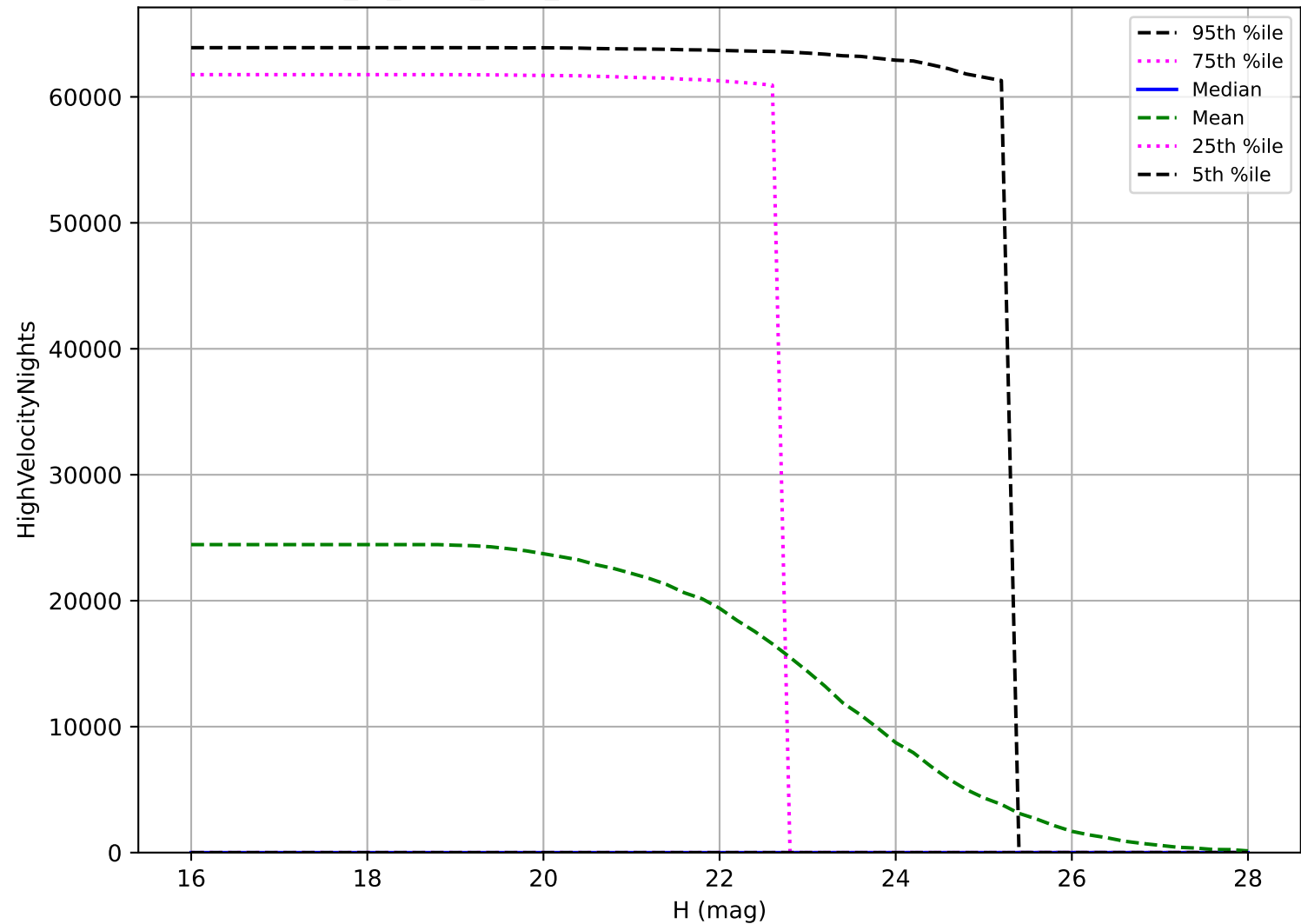
extra_ss_neo7_v3.4_10yrs: PHA High velocity pair detection loss
