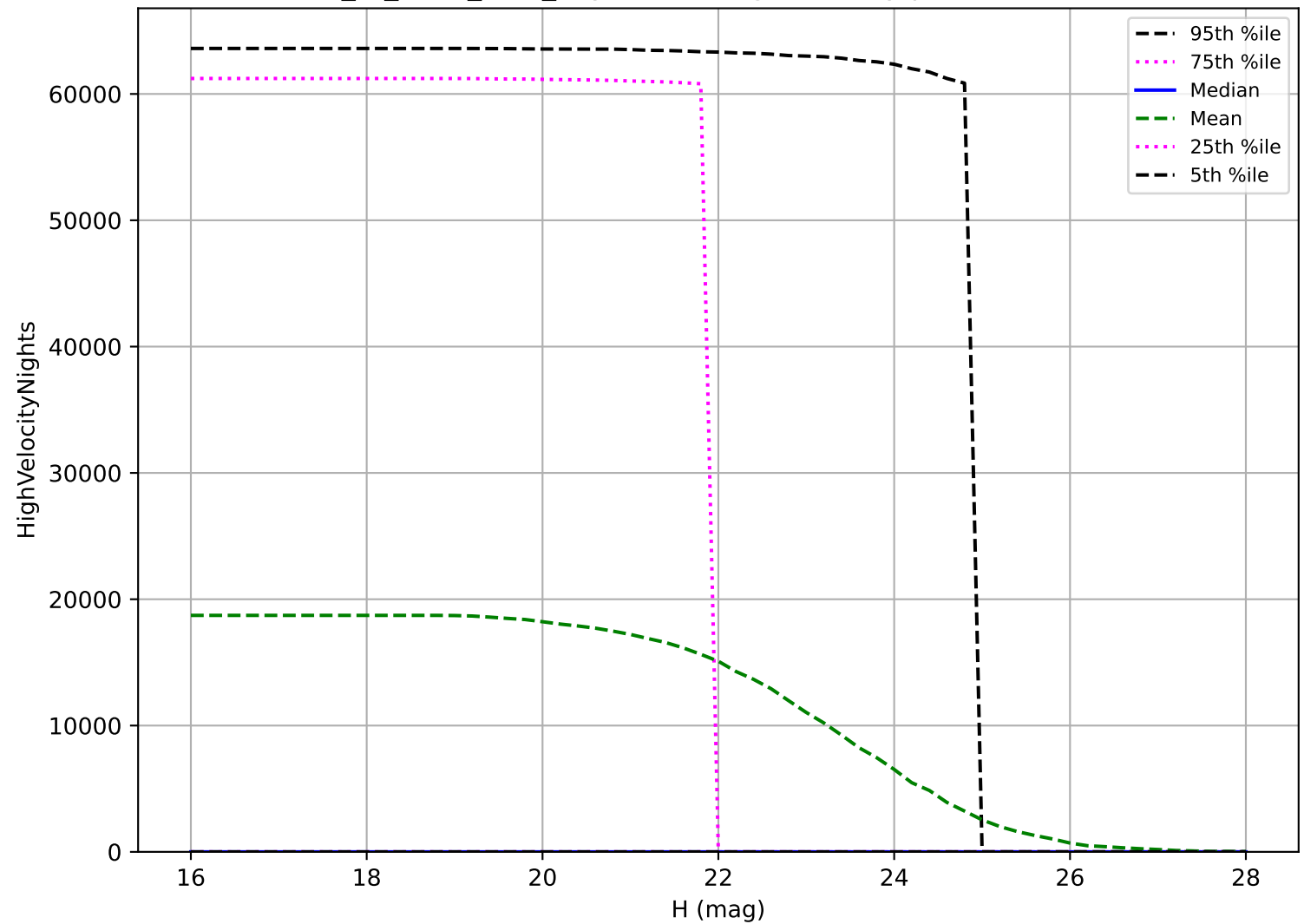
extra_ss_neo7_v3.4_10yrs: NEO High velocity pair detection loss
