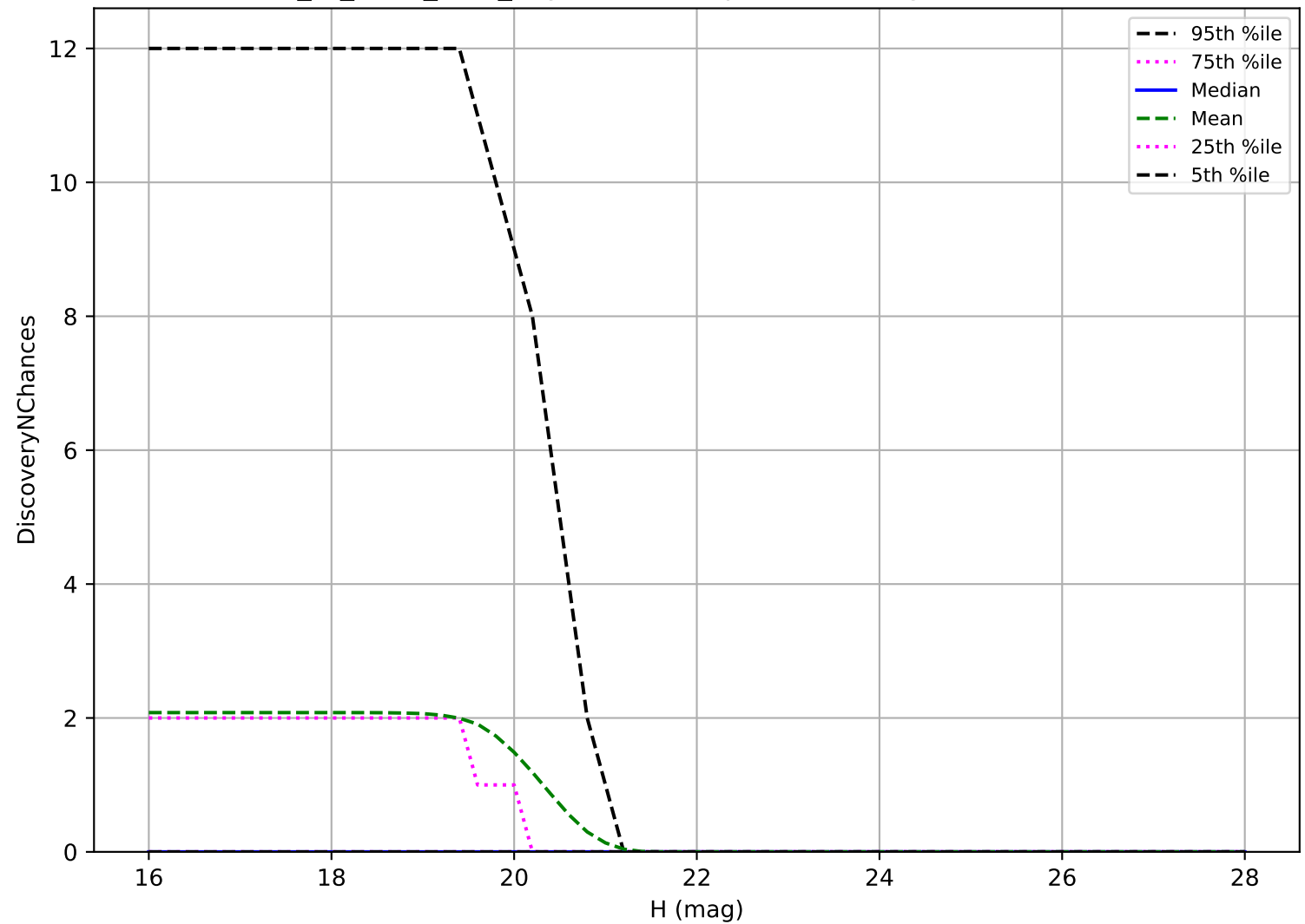
extra_ss_neo7_v3.4_10yrs: Vatira 3 pairs in 15 nights detection loss
