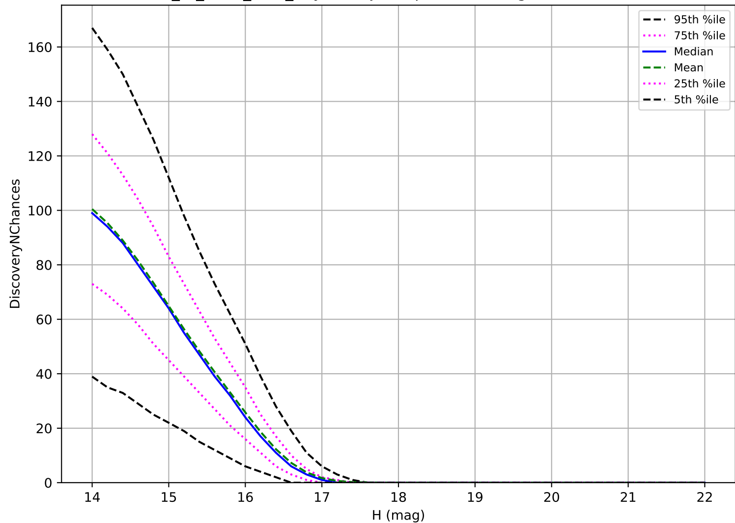
extra_ss_neo7_v3.4_10yrs: Trojan 3 pairs in 15 nights detection loss
