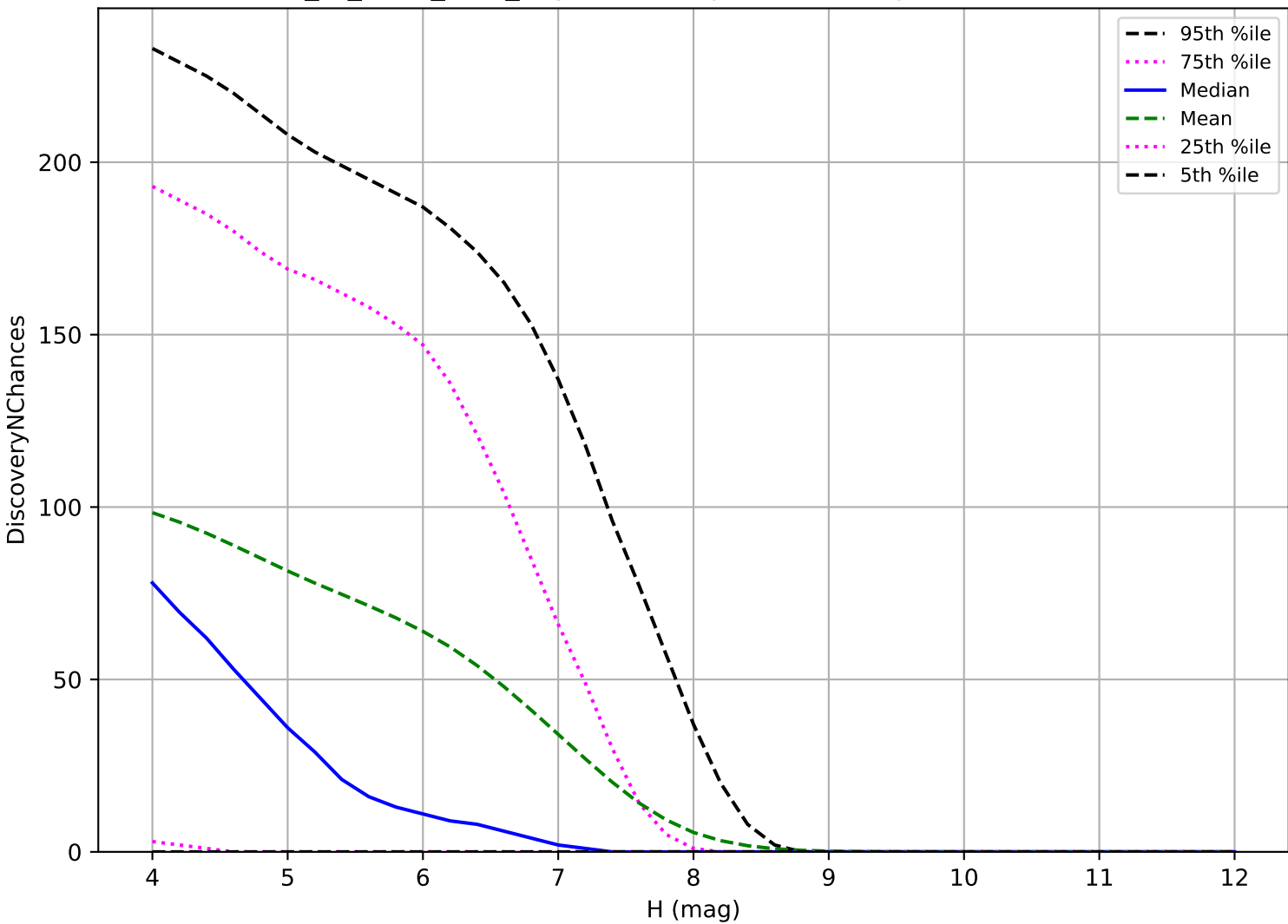
extra_ss_neo7_v3.4_10yrs: TNO 3 pairs in 15 nights detection loss
