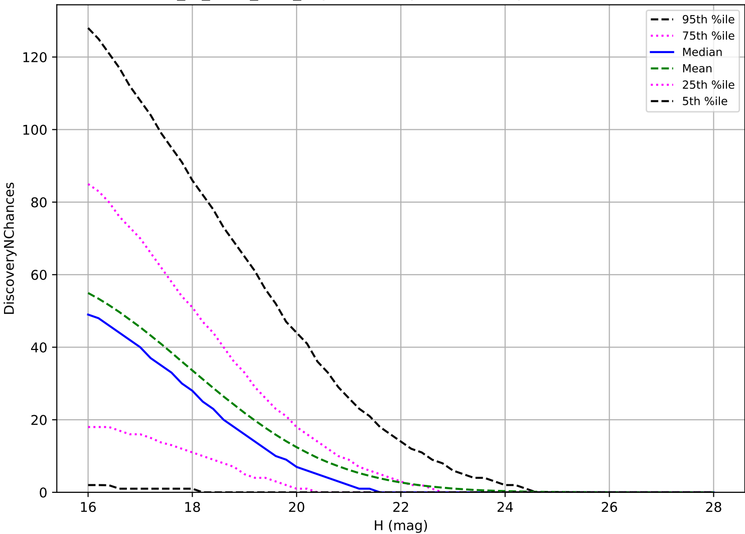
extra_ss_neo7_v3.4_10yrs: PHA 3 pairs in 15 nights detection loss
