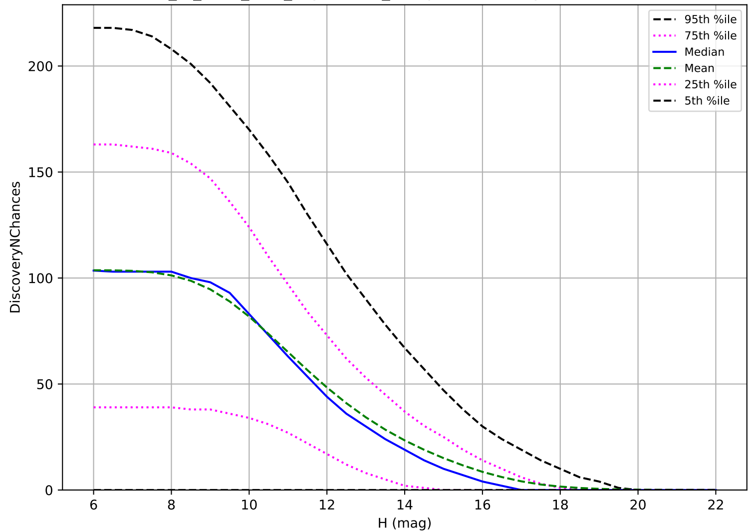
extra_ss_neo7_v3.4_10yrs: OCC_r5 3 pairs in 15 nights detection loss
