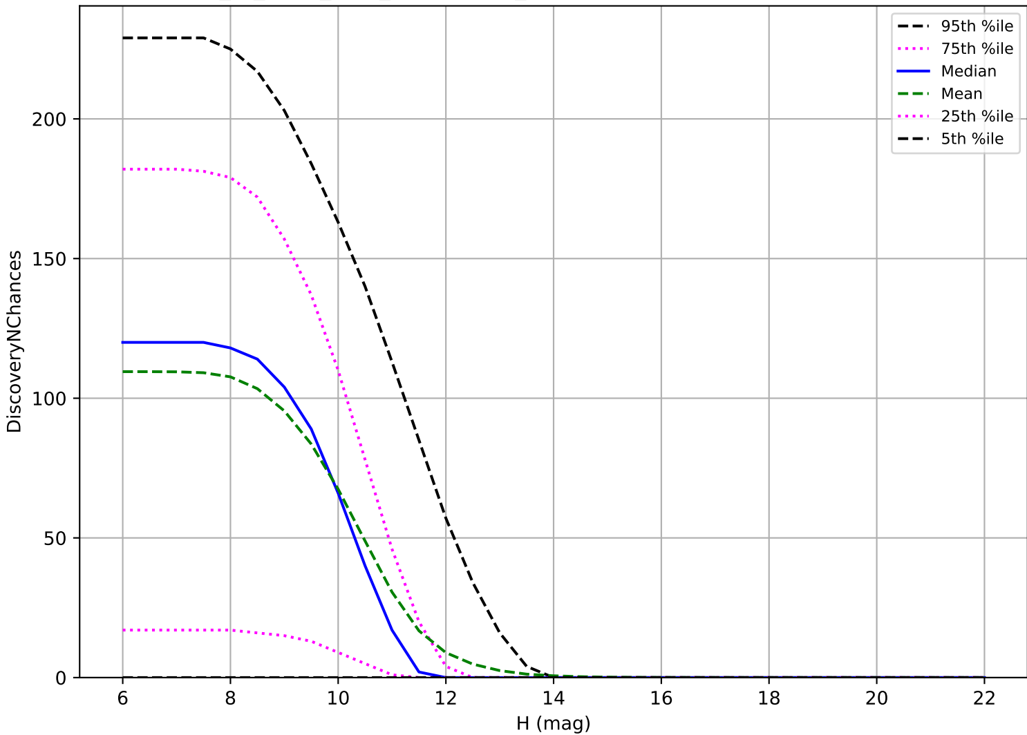
extra_ss_neo7_v3.4_10yrs: OCC_r20 3 pairs in 15 nights detection loss
