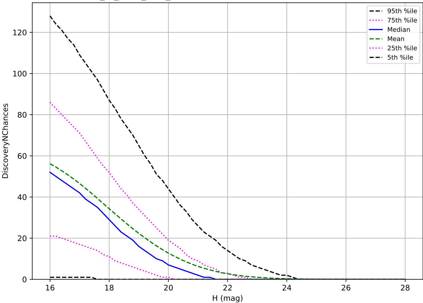
extra_ss_neo7_v3.4_10yrs: NEO 3 pairs in 15 nights detection loss
