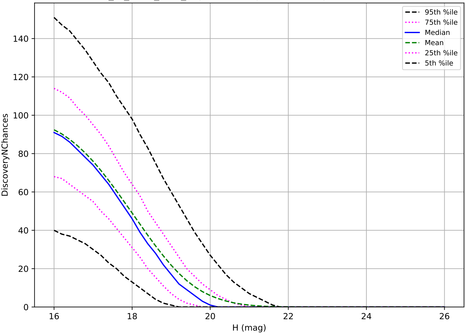
extra_ss_neo7_v3.4_10yrs: MBA 3 pairs in 15 nights detection loss
