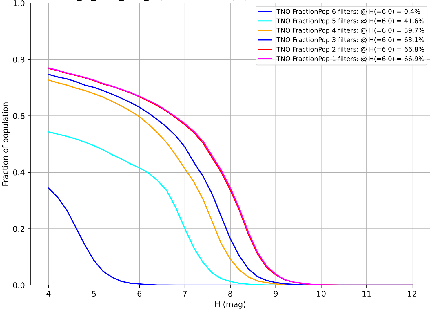
extra_ss_neo7_v3.4_10yrs: Fraction of population with colors in X filters TNO
