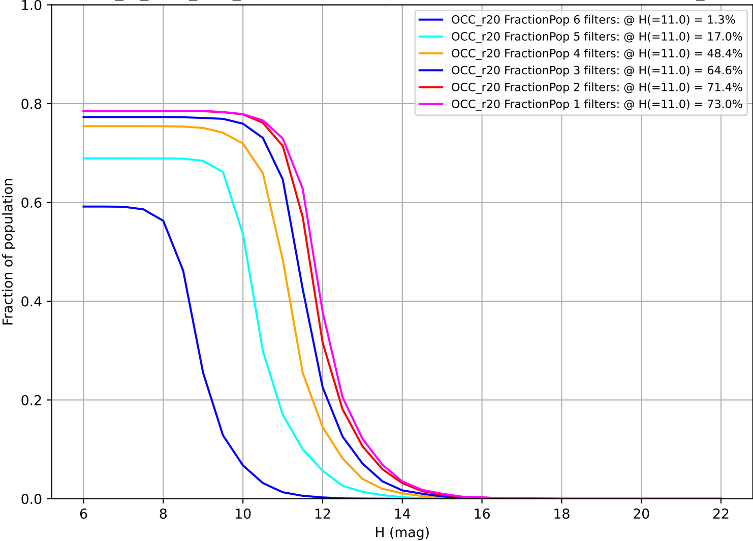
extra_ss_neo7_v3.4_10yrs: Fraction of population with colors in X filters OCC_r20
