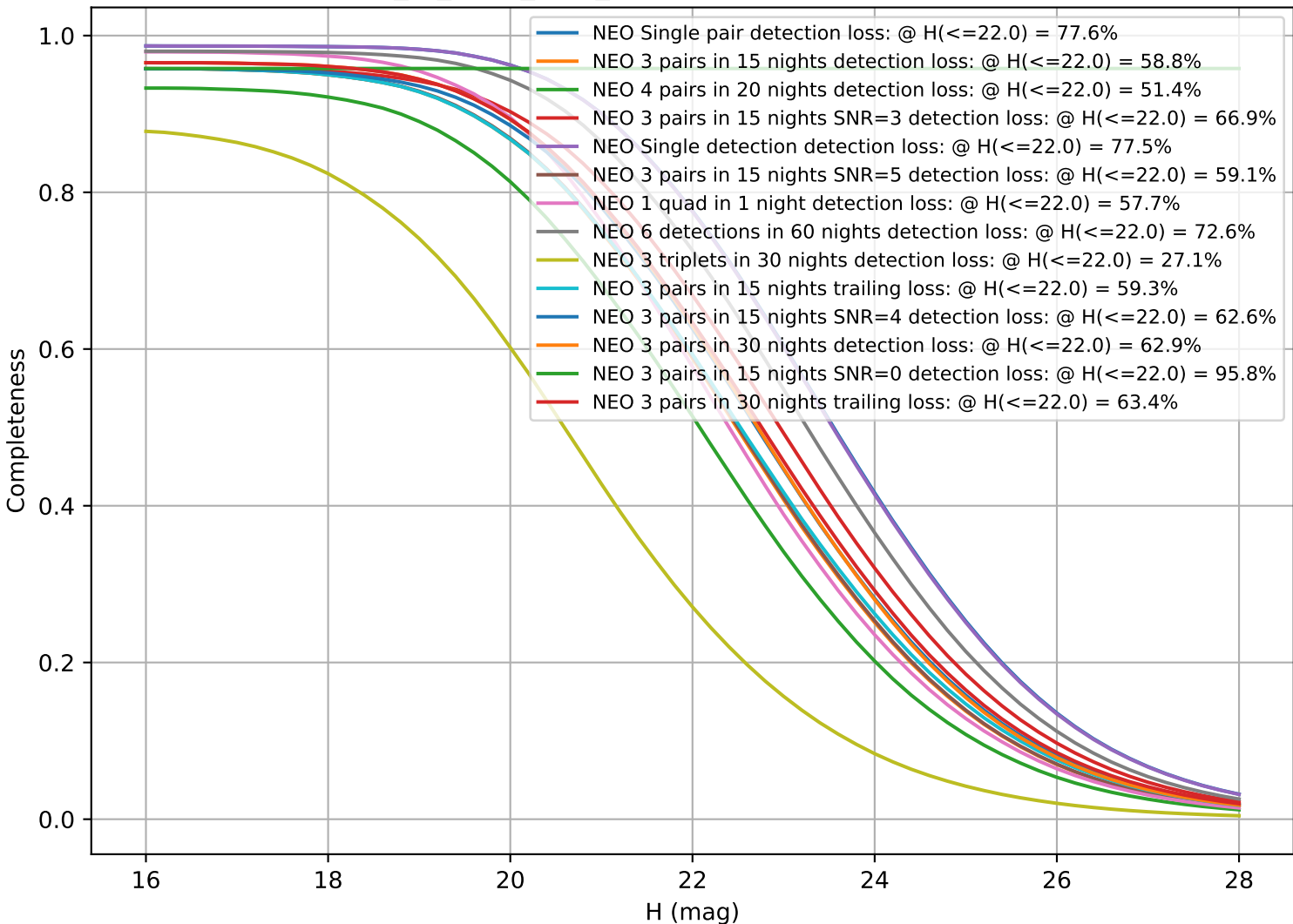
extra_ss_neo7_v3.4_10yrs: CumulativeCompleteness
