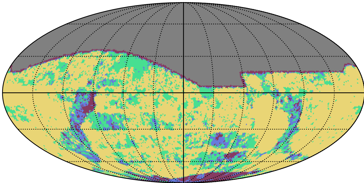
extra_ss_neo7_v3.4_10yrs g band: YearCoverage night
