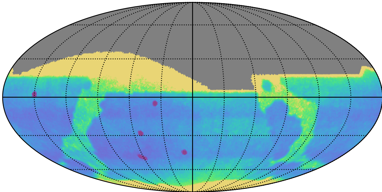
extra_ss_neo7_v3.4_10yrs : Proper Motion Uncert @ 24.0
