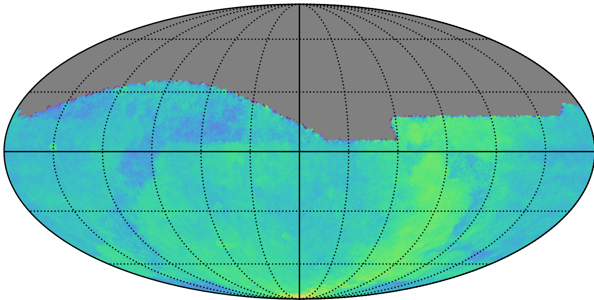
extra_ss_neo7_v3.4_10yrs : Parallax Coverage @ 24.0
