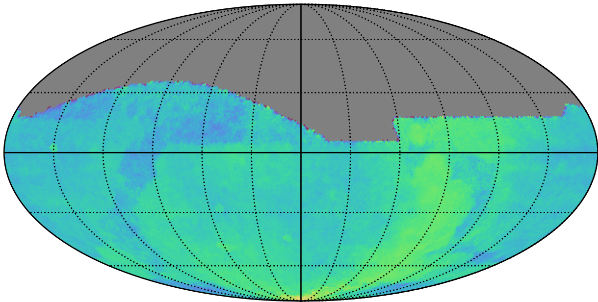
extra_ss_neo7_v3.4_10yrs : Parallax Coverage @ 22.4
