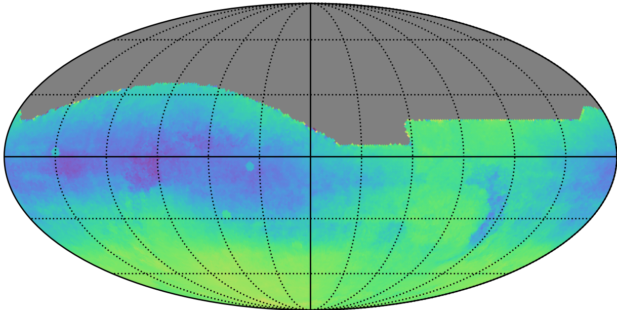
extra_ss_neo7_v3.4_10yrs : Parallax-DCR degeneracy @ 22.4
