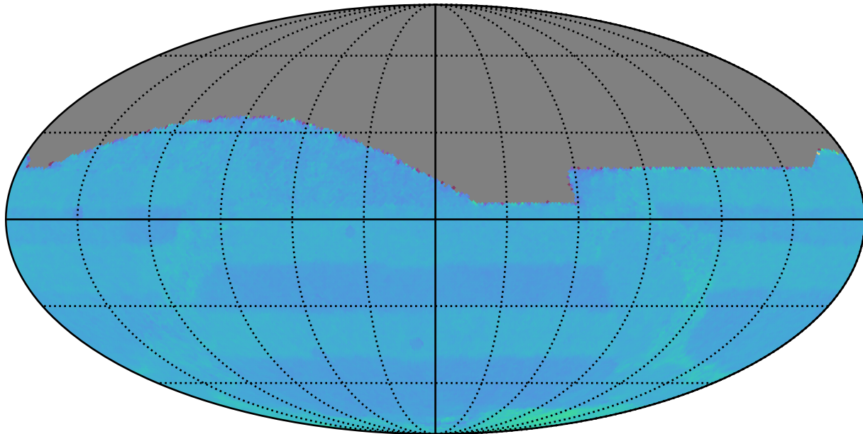
extra_ss_neo7_v3.4_10yrs : Normalized Proper Motion Uncert @ 20.5
