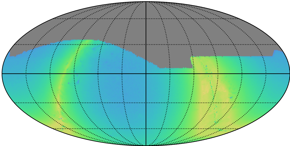
extra_ss_neo7_v3.4_10yrs r: N stars to Precision 0.20
