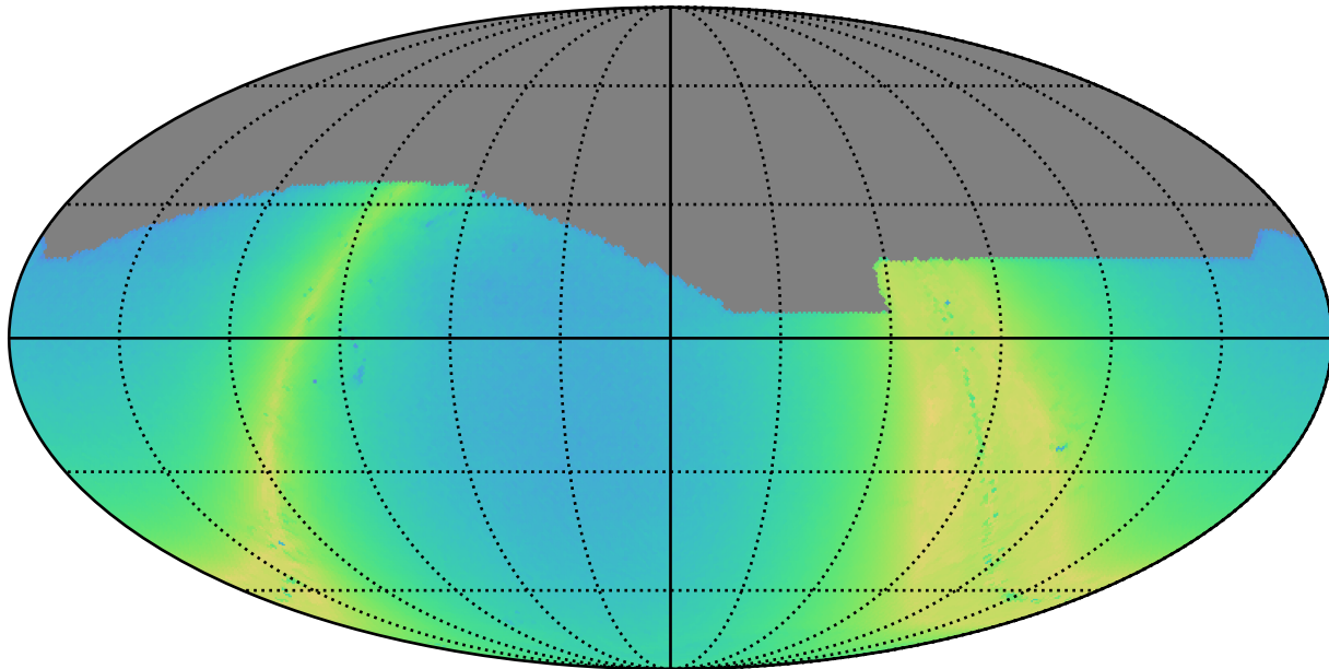
extra_ss_neo7_v3.4_10yrs i: N stars to Precision 0.20
