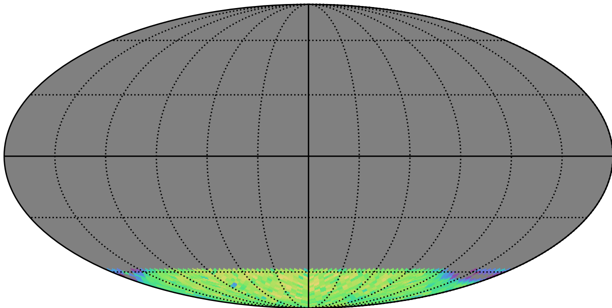
extra_ss_neo7_v3.4_10yrs gi SCP: LVDwarfs
