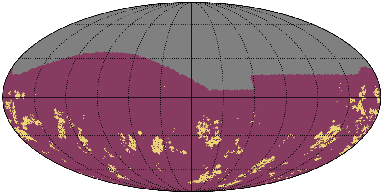
extra_ss_neo7_v3.4_10yrs g band: Gaps_7hr
