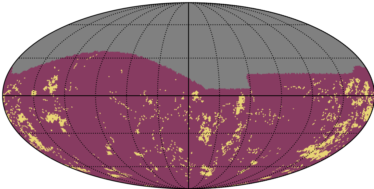
extra_ss_neo7_v3.4_10yrs g band: Gaps_3hr
