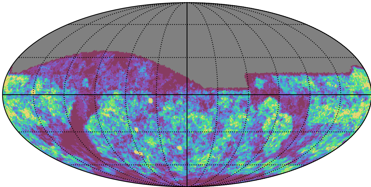
extra_ss_neo7_v3.4_10yrs g band: Gaps_24hr
