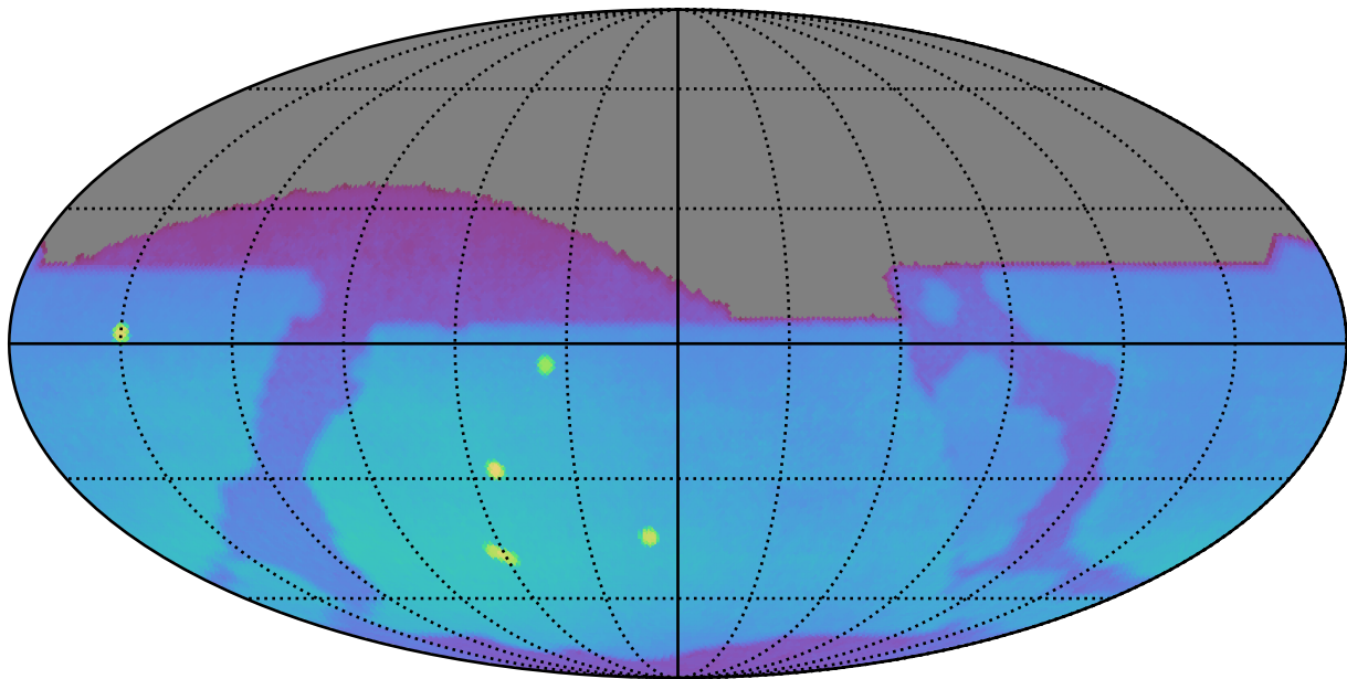
extra_ss_neo7_v3.4_10yrs : Brown Dwarf, L7
