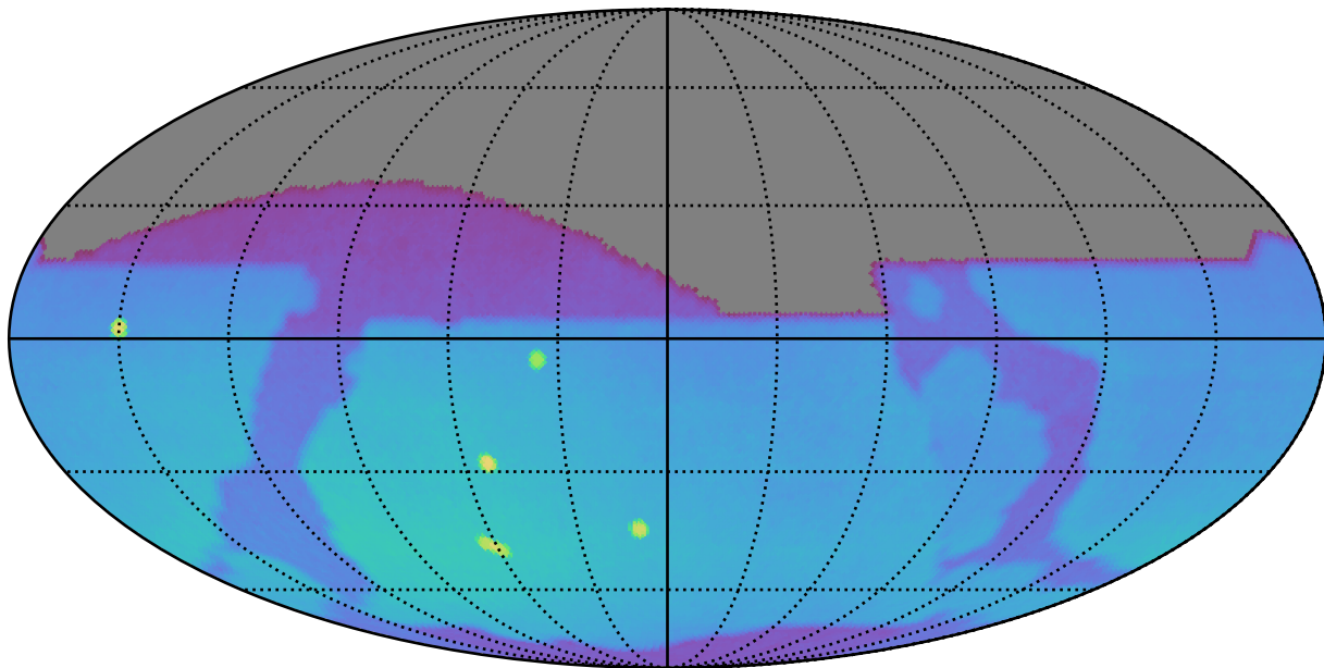
extra_ss_neo7_v3.4_10yrs : Brown Dwarf, L4
