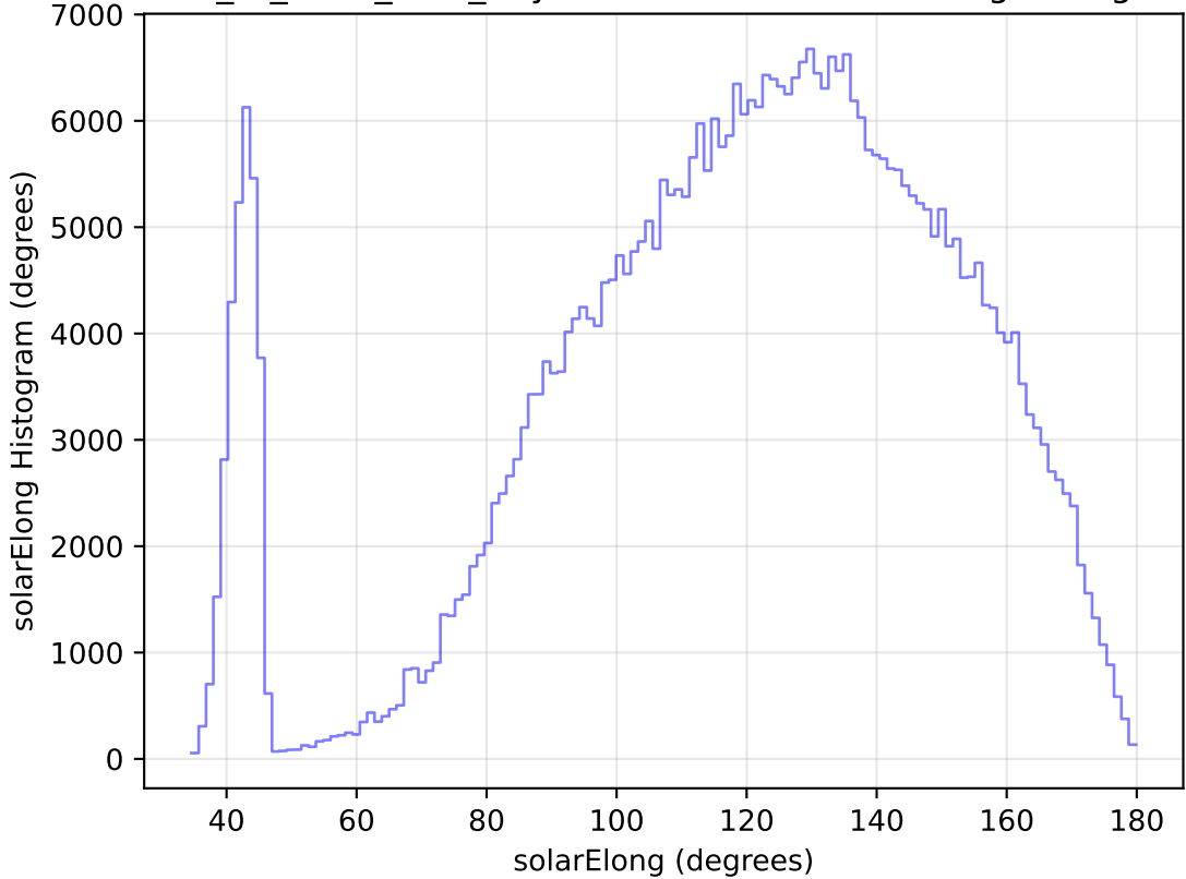
extra_ss_neo7_v3.4_10yrs WFD z band: solarElong Histogram
